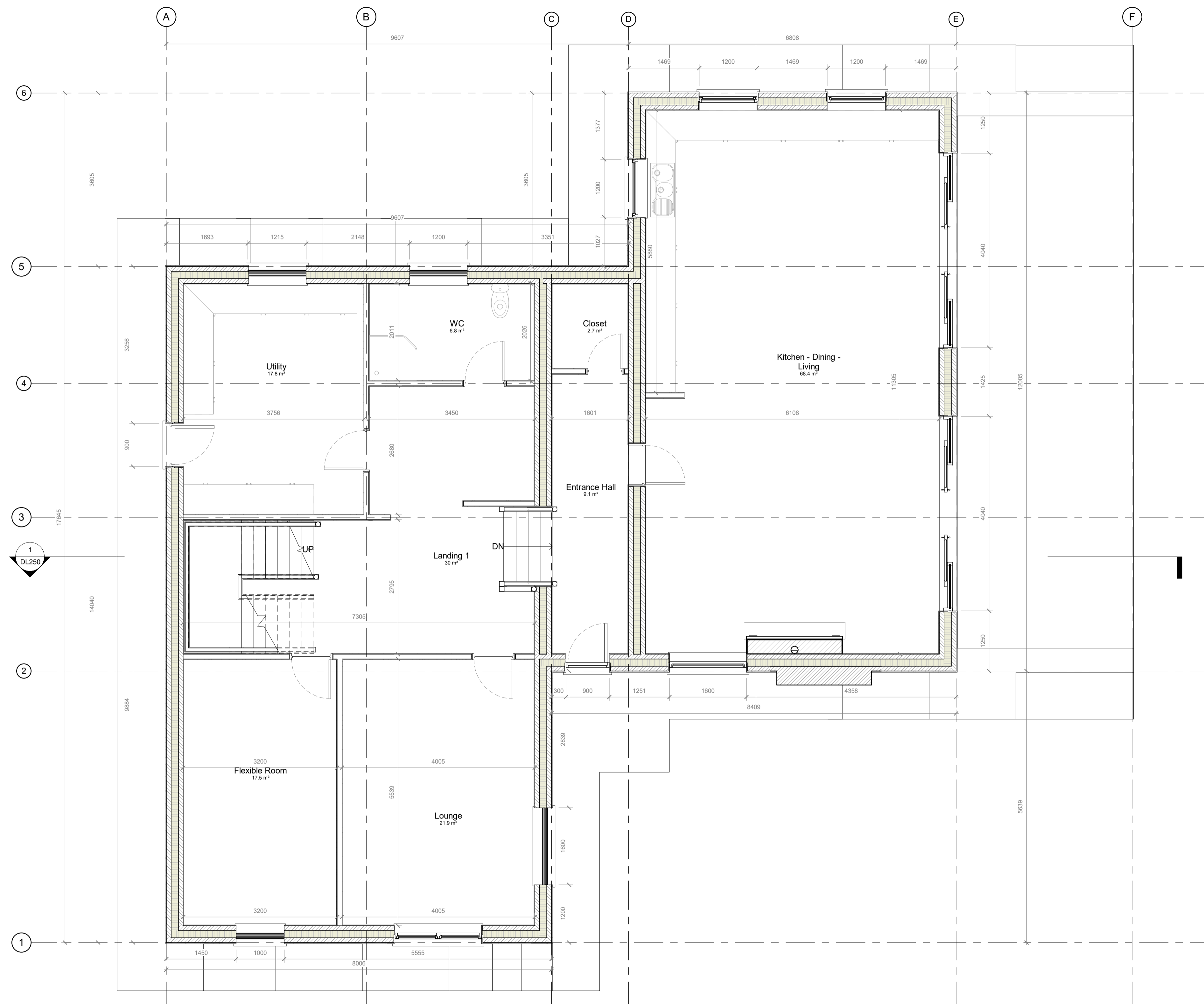
01_Ground Floor Plan 1 : 50
